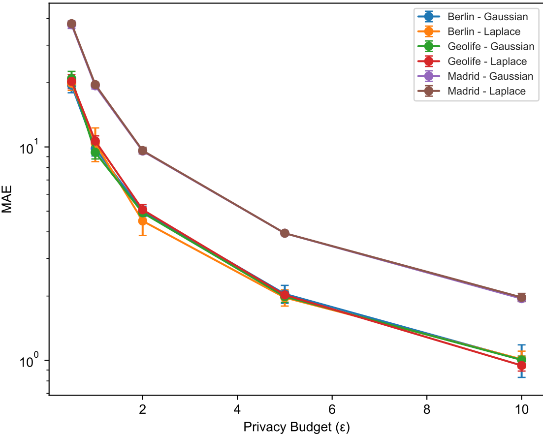
Mechanism Performance (visits_per_tile, M=10)
