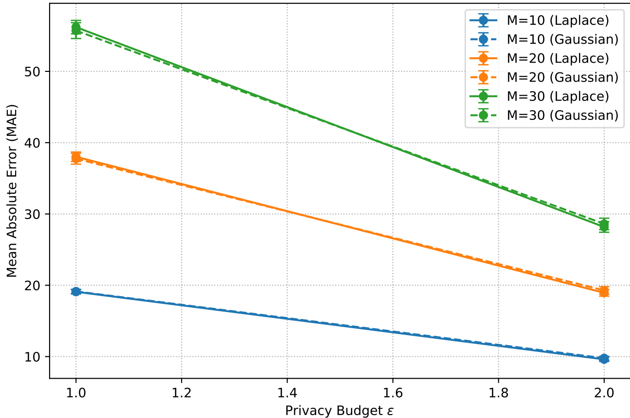
M-Clipping Parameter Scaling Analysis (Madrid, visits per tile)
