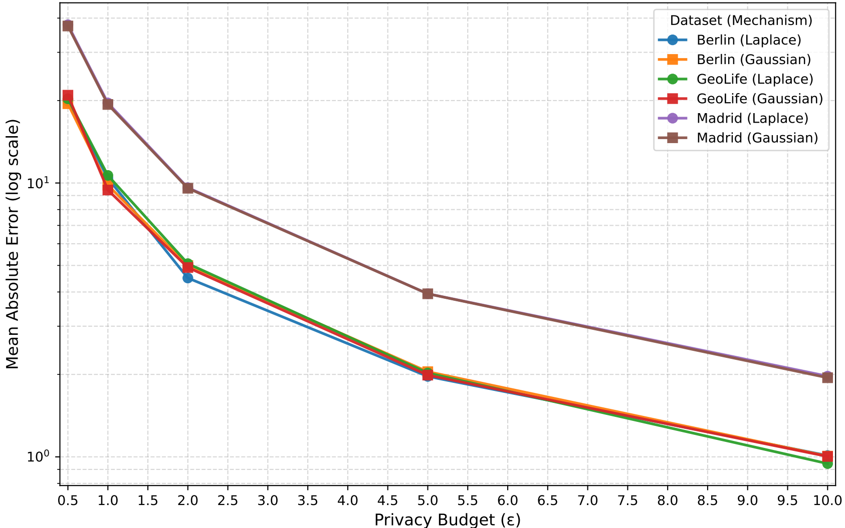
Privacy Budget Scaling: Laplace vs. Gaussian
