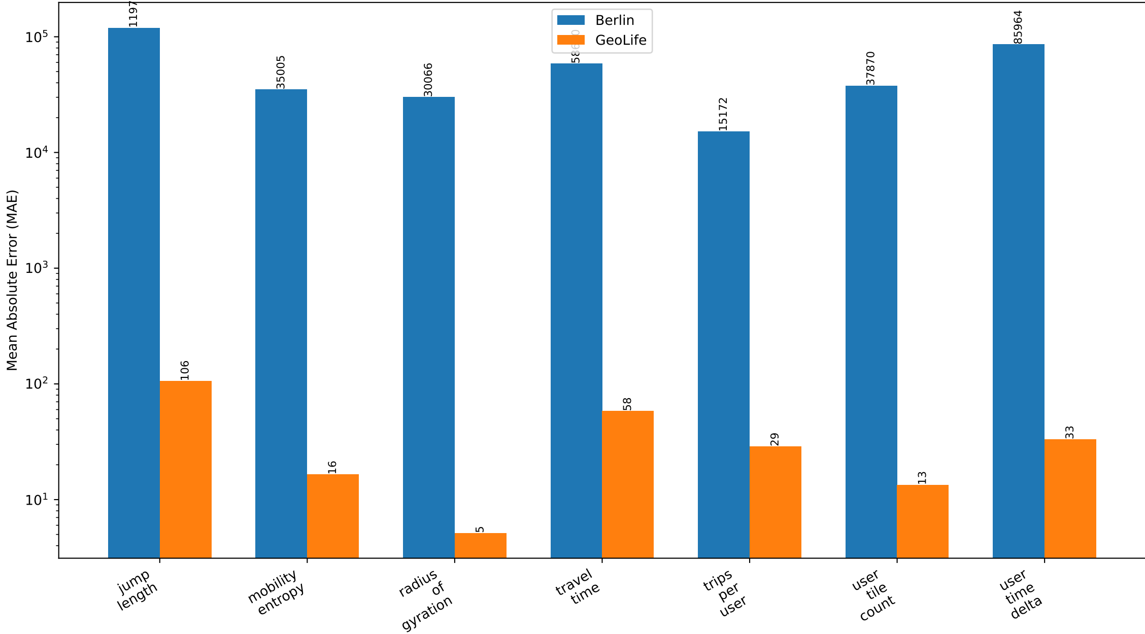
Analysis Sensitivity Ranking: Berlin vs GeoLife (log MAE, \epsilon=1.0 , M=10 )
